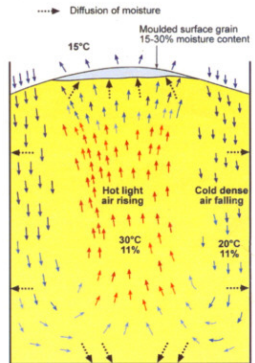
Diagram 1. Natural convection currents are formed by displacement of hot air by dense coldair. Adapted from H.J.Griffith (1964) 'Bulk storage of grain', CSIRO
